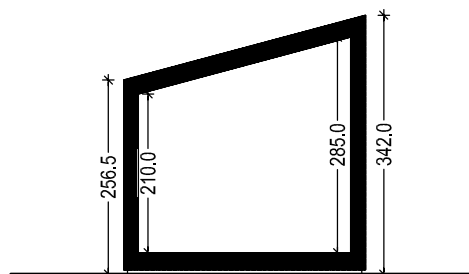
Snit
